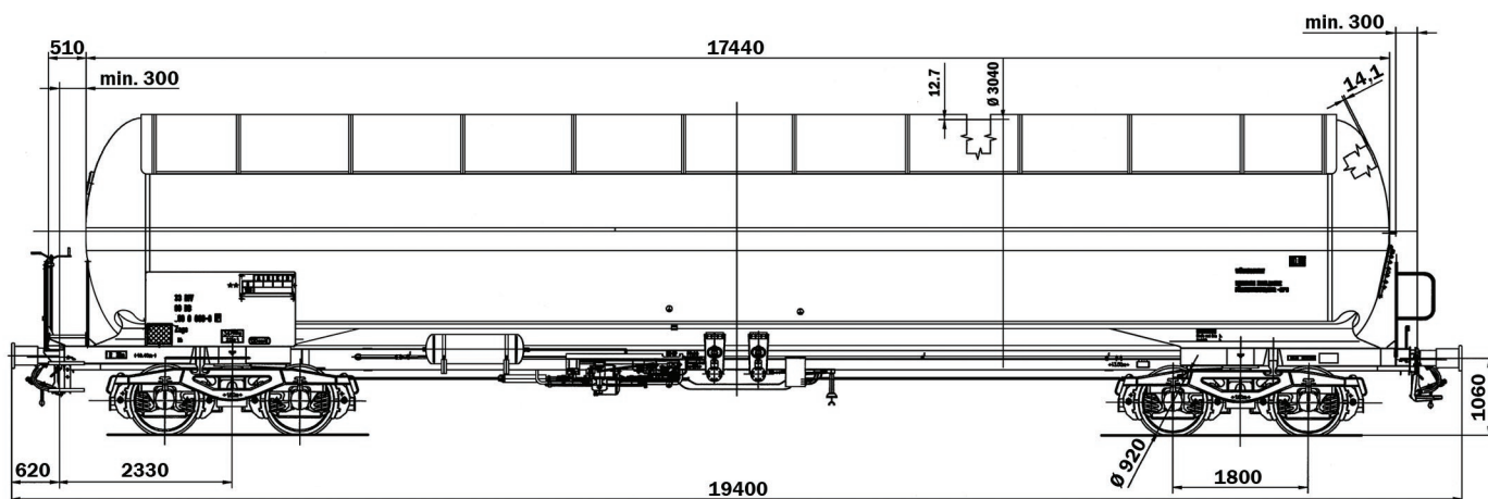
Wagon gauge UIC 505-1
