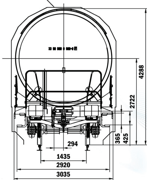
Wagon gauge UIC 505-1
